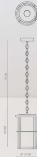
Arbor Round Pendant PL-106002 E27 1x40W Textured Black IP23
