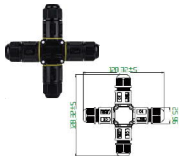
IP Connectors 4 Way Connector IP Rating - IP68
